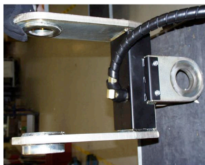
KNV load cell for the grab device
